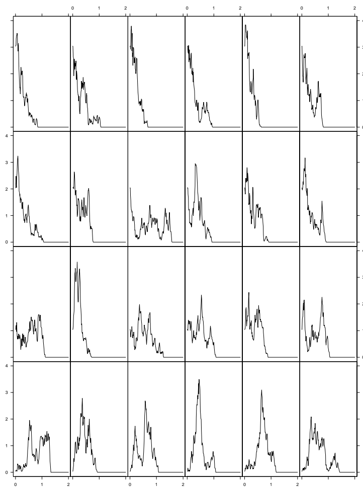
Figure 1 Simulated trajectories of the local time process of a reflecting Brownian bridge of length 1. Each panel shows an exact computer simulation of the height profile of a uniform random forest of k rooted trees with n = 2500 vertices, generated from binomial random variables via Lemma 9, and scaled as in (15) to approximate (X_{\ell,1,v}, v \geq 0) governing the local times of a reflecting Brownian bridge of length 1 given local time \ell at 0. In each panel, v ranges from 0 to 2 on a horizontal scale, and the vertical scale for local time ranges from 0 to 4. The area under each trajectory differs from negligibly from 1. Each row shows 6 repetitions for a given initial value \ell = 2k/\sqrt{n} = k/25 , with \ell = 1/25 in the bottom row approximating the local time process of a Brownian excursion, and \ell = 1, 2, 3 in rows above.
